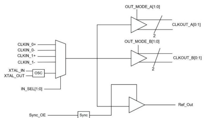
Figure 1 Functional Diagram
